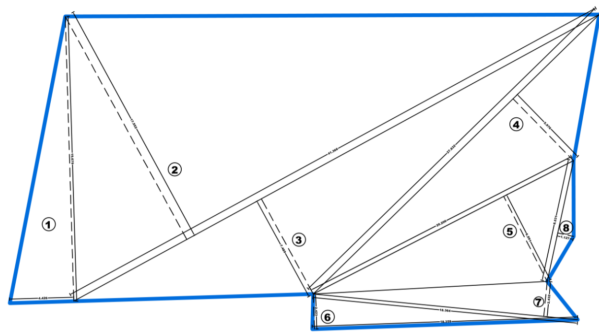
PLOT AREA DIAGRAM SCALE - 1:250
